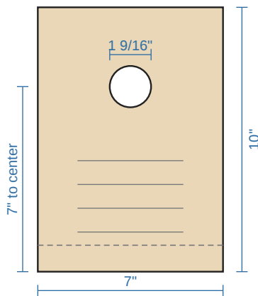
D Front: 1 9/16" Round Hole
